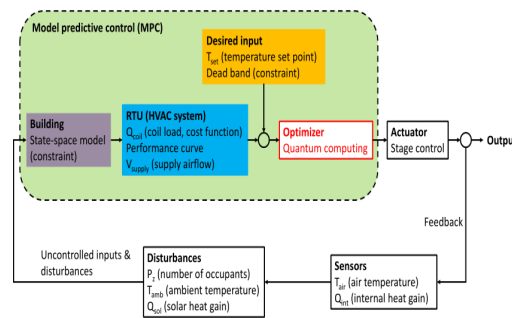
Figure 3: Basic Quantum MPC
