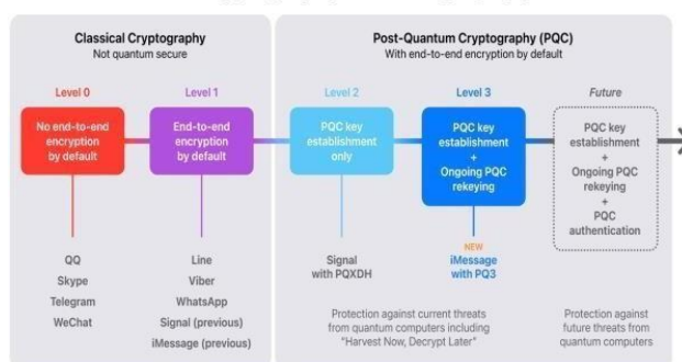
Figure 2: PQC, or post-quantum cryptography
