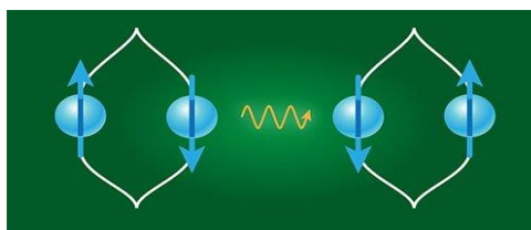
Figure 1: Conceptual Diagram of Entangled Qubit States
